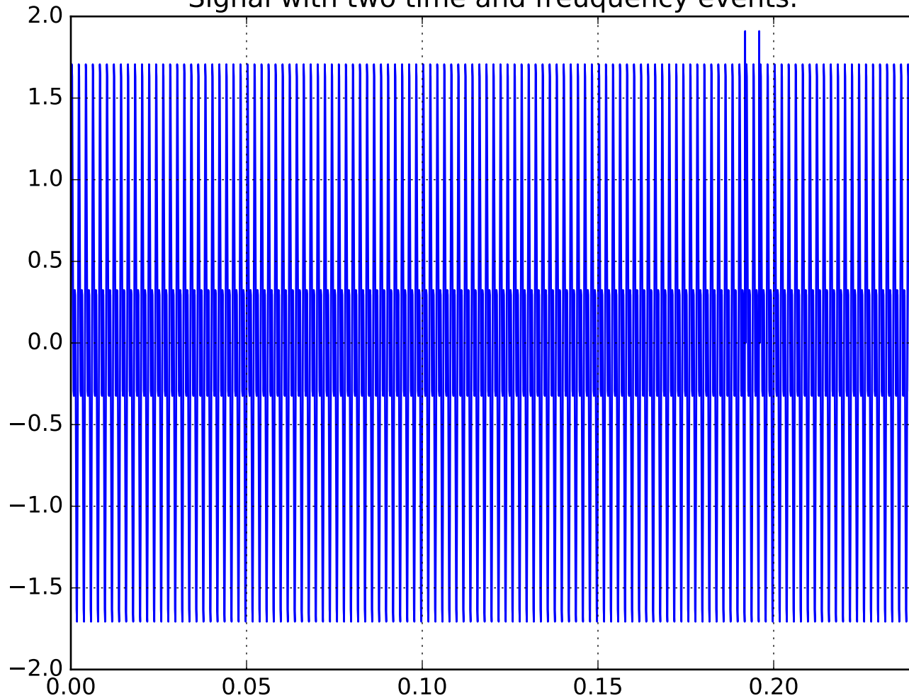
Signal with two time and frequency events.
